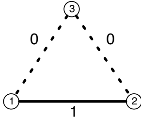
FIGURE 1. A generalized edge random graph that is not an edge random graph.
