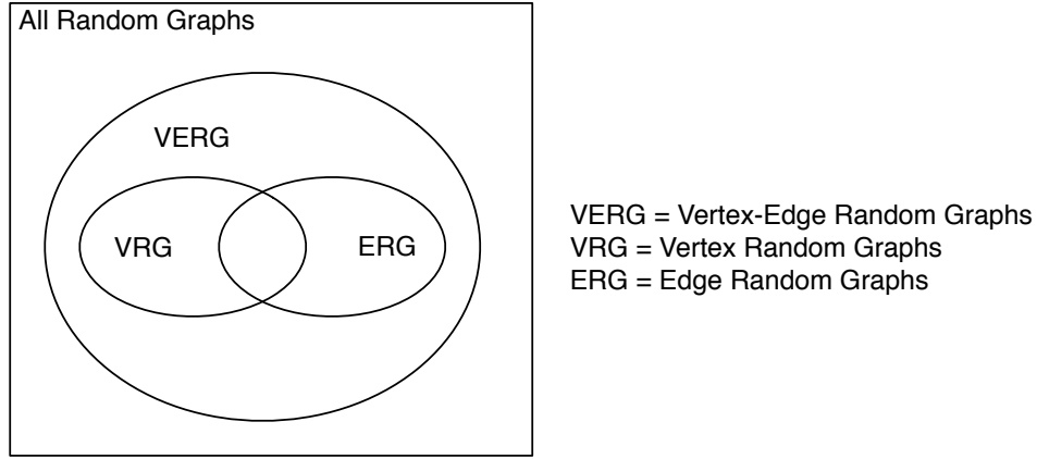
FIGURE 2. Venn diagram of random graph classes. The results of this paper show that all five regions in the diagram are nonempty.
